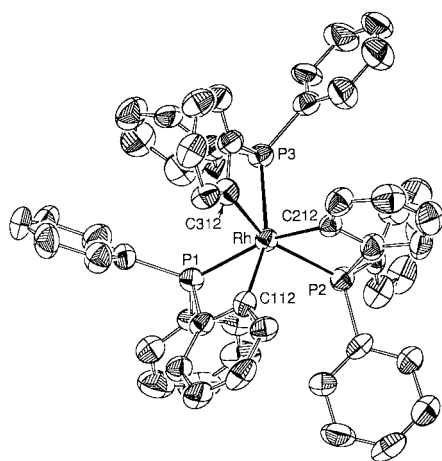
Fig. 2 Molecular structure of [\text{Rh}\{\text{C}_6\text{H}_4(\text{PPh}_2)\text{-}2\}_3]\cdot\text{CHCl}_2 25 . Ellipsoids represent 50% probability levels.
